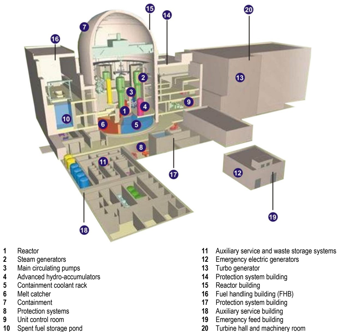
Fig. II.10: Layout of the ATMEA1 unit
