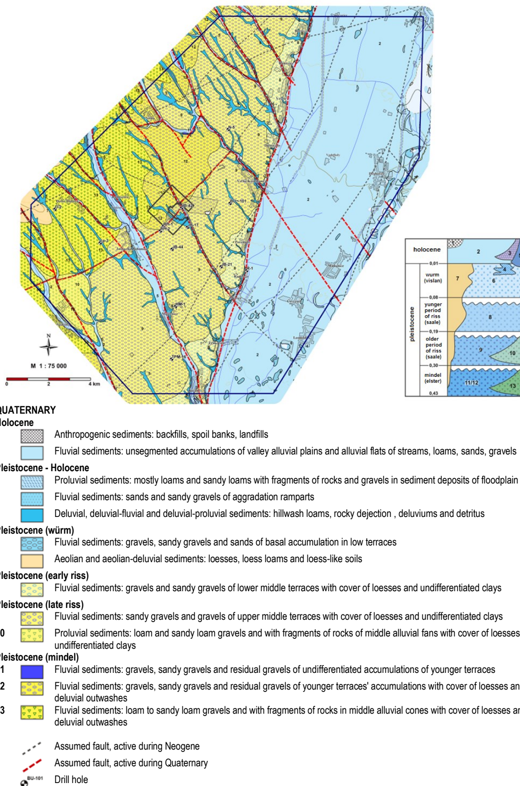
Fig. III.12: Geological map of the NNPP surroundings
