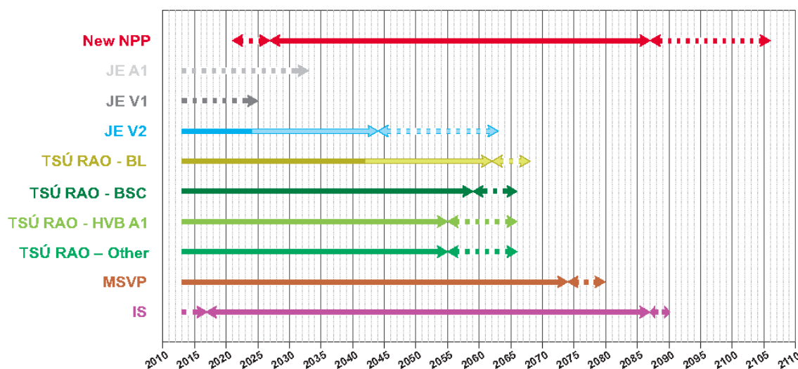
Fig. II.18: Course of concurrent impacts of the individual nuclear facilities at the Jaslovské Bohunice site
