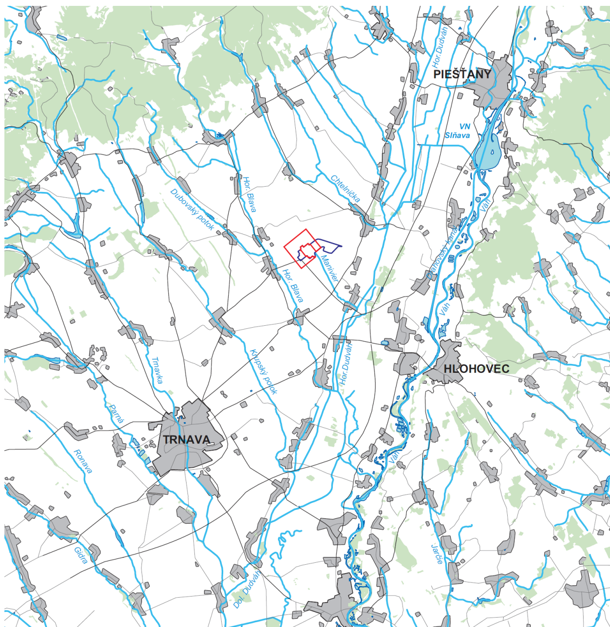
Fig. III.8: Water streams and water areas in the wider area of Jaslovské Bohunice
